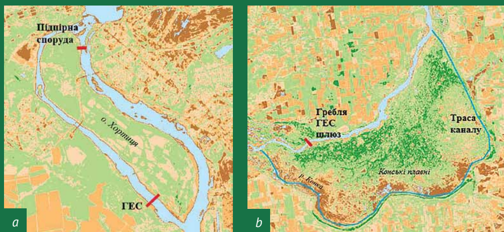
Options for the construction of small hydropower plants (based on a presentation by Dmytro Stefanyshyn [349] ): a) on the main channel of the Dnipro River in the vicinity of Khortytsia Island; and b) on an embanked section of the Dnipro River downstream of the Koneski Plavni wetlands, with the construction of a bypass channel.
